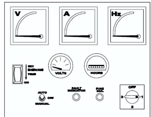
Generac CMA Liquid Cooled Control Panel
